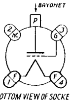
BOTTOM VIEW OF SOCKET
