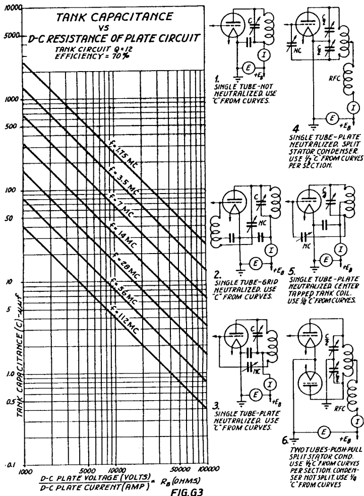
FIG. G3 For push-pull output, whether the tank is split or not, the load impedance is two times as great so that the total capacitance must be reduced to 1/2 the reference value. The capacitance per section is therefore the same as the total capacitance for a single ended grid neutralized stage of the same input power. However, the push-pull stage will have twice the power input and half the R B of the single ended stage and if the capacitance is calculated using the R B of the push-pull stage, the result must be again divided by 2. For a single-ended plate neutralized amplifier, with a center-tapped tank coil, the load is quadrupled, therefore the total capacitance is 1/4 and the capacitance per section is 1/2 the total capacitance for the reference case. If
