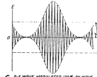
C R-F WAVE MODULATED 100% BY WAVE SHOWN IN "A", WITH DISTORTION PEAKS UPWARD
