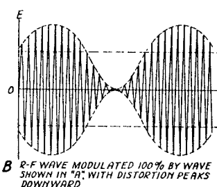
A MODULATING WAVE CONTAINING FUNDAMENTAL AND 15% 2ND HARMONIC
