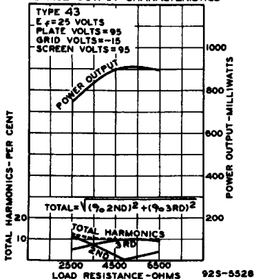
AVERAGE OUTPUT CHARACTERISTICS
