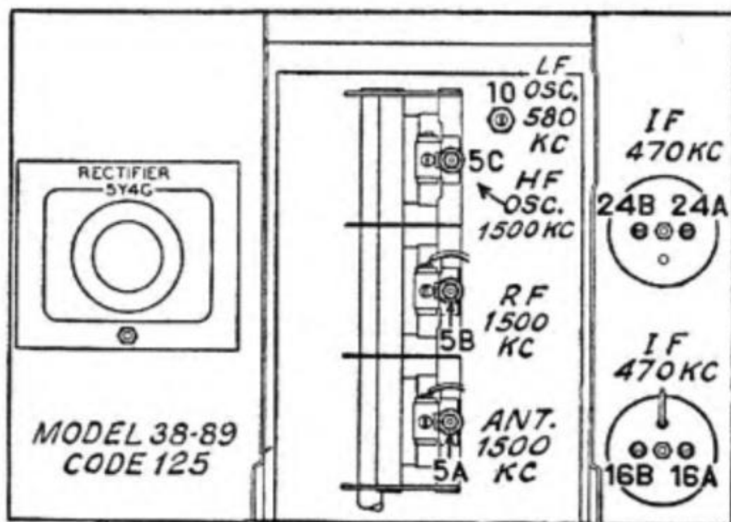
LOCATION OF TRIMMERS. TOP OF CHASSIS
