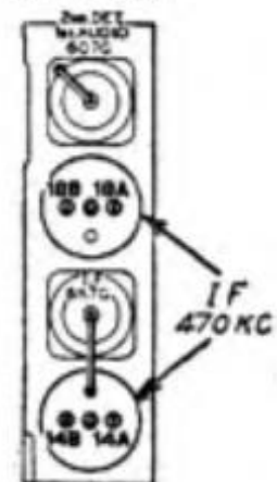
MODEL 38-60 CODE 125 TOP VIEW
