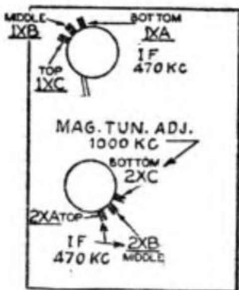
PARTIAL TOP VIEW MODEL 38-2, CODE 121 RUN # 2
