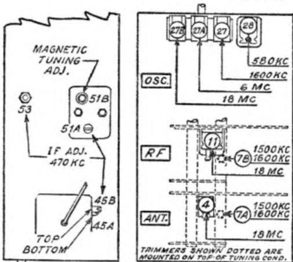
MODEL 38-3 - CODE 121 IF TRIMMERS TRIMMER VIEW TOP OF CHASSIS UNDERSIDE OF CHASSIS
