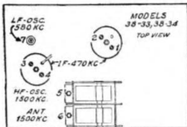
Locations of Components—Top of Chassis
